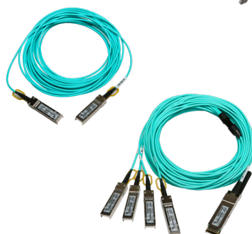
Intel Ethernet SFP28 AOC and QSFP28 to SFP28 AOC
